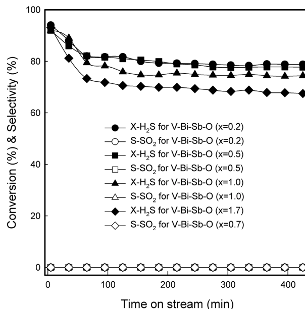
Fig. 2. Time variant conversion of \text{H}_2\text{S} and selectivity to \text{SO}_2 for \text{Bi}_4\text{V}_{2-x}\text{Sb}_x\text{O}_{11-y} catalysts at 260 °C ( \text{H}_2\text{S}/\text{O}_2/\text{NH}_3/\text{H}_2\text{O}/\text{He}=5/2.5/5/60/27.5 , GHSV=12,000 \text{h}^{-1} ).
