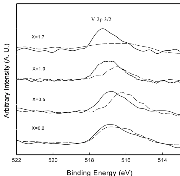
Fig. 5. XPS analyses of V 2p 3/2 for Bi 4 V 2-x Sb x O 11-y catalysts before (solid line) and after (dashed line) the reaction: Reaction condition (H 2 S/O 2 /NH 3 /H 2 O/He=5/2.5/5/60/27.5, GHSV=12,000 h -1 ).
